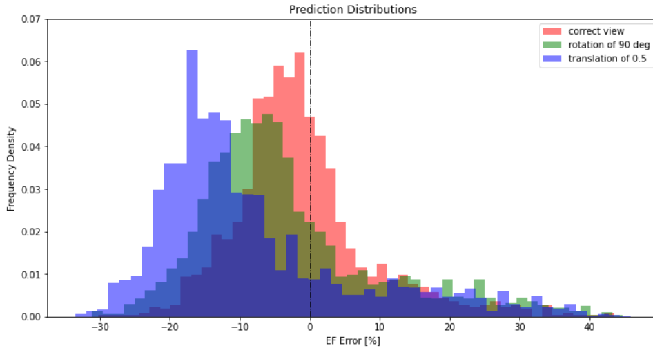
Fig. 5. EF Error distribution for best view, 90 degrees of rotation, and a translation of 0.5.
