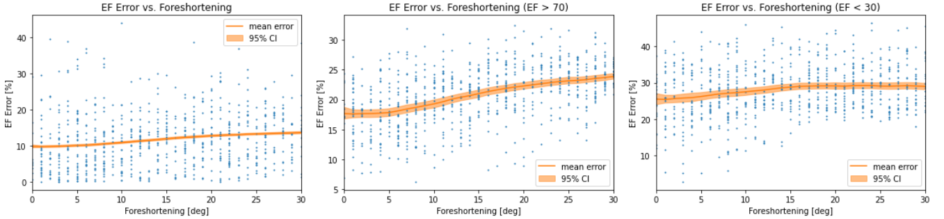
Fig. 8. Performance figures for slices with introduced foreshortening.
