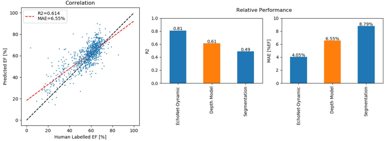
Fig. 7. Performance of depth map model and comparison to prior works
