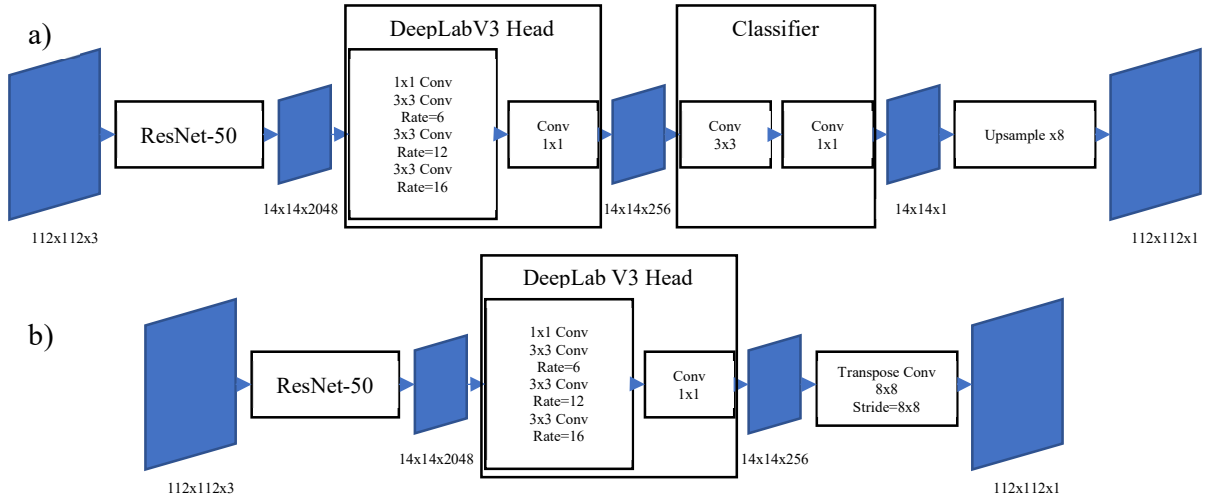
Fig. 3. a) Original DeepLabV3 architecture b) architecture used here
