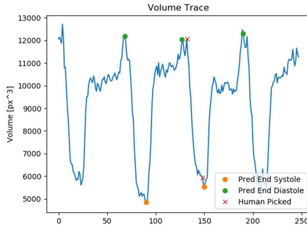
Fig. 9. Example predicted volume tracing
